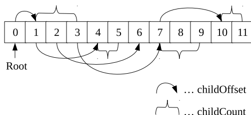
Figure 4.1.3: Example FlatTree
