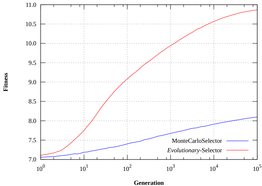
Figure 2.8.1: Selector-performance (Knapsack)
