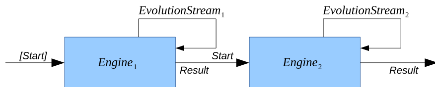
Figure 4.1.5: Engine concatenation
