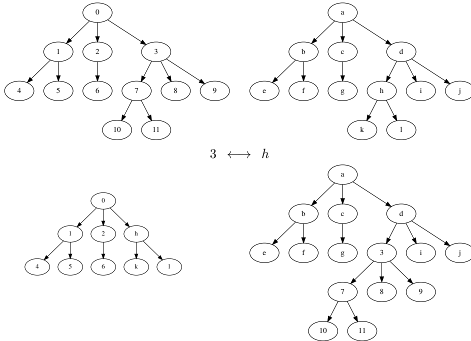
Figure 4.1.4: Single-node crossover
