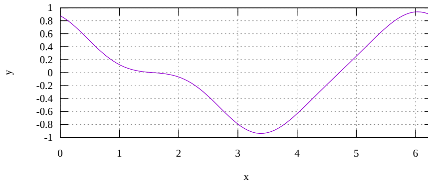
Figure 5.2.1: Real function
