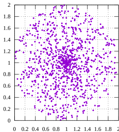
Figure 4.1.8: Circle points
