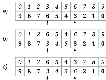
Figure 1.3.11: Partially-matched crossover
