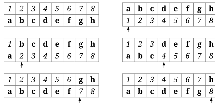
Figure 1.3.8: Single-point crossover
