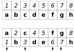
Figure 1.3.12: Uniform crossover
