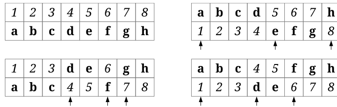
Figure 1.3.10: 3-point crossover
