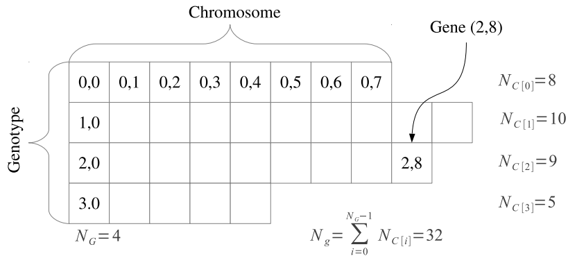
Figure 1.3.2: Genotype structure
