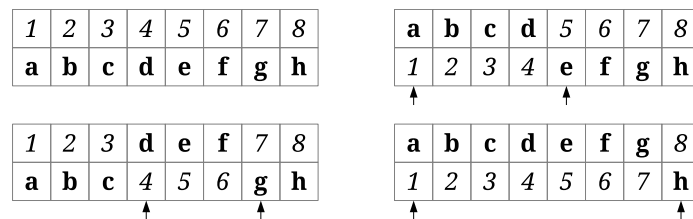
Figure 1.3.9: 2-point crossover
