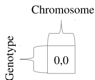
Figure 1.3.5: Genotype scalar
