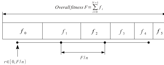
Figure 1.3.7: Stochastic-universal selection
